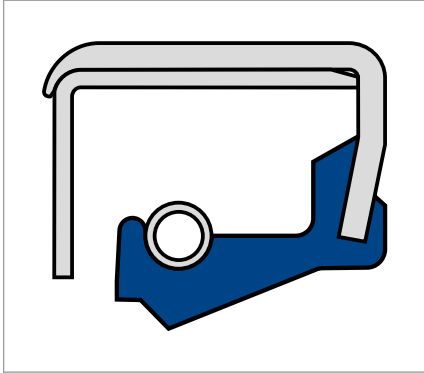
Simmerring B2...
